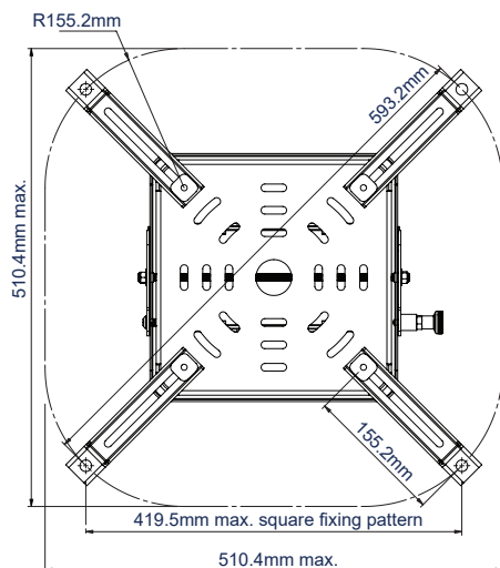
BOTTOM VIEW WITH INCLUDED SHORT EXTENSION LEGS
